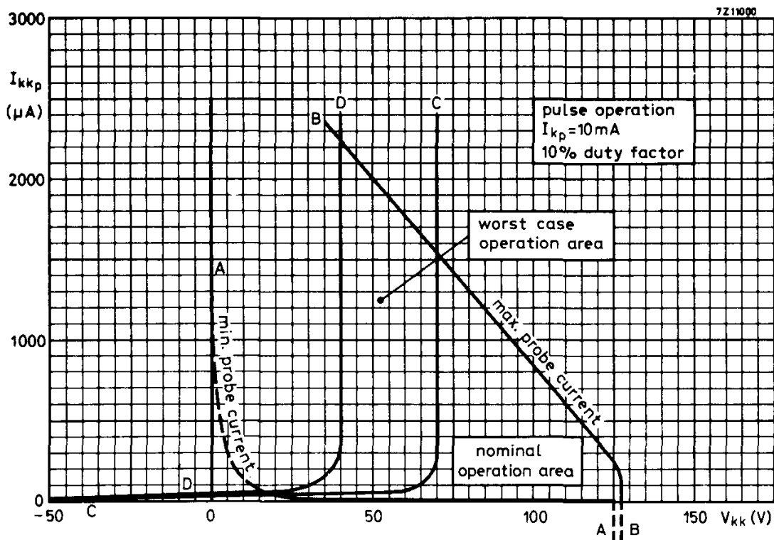
PEAK PROBE CURRENT TO INDIVIDUAL NON-CONDUCTING CATHODES
