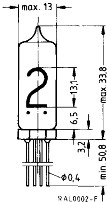
RAL0002-F Dimensions in mm
