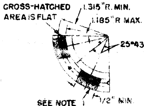
SEE NOTE 1 DETAIL OF BOTTOM VIEW OF JUMBO ANNULAR BASE
