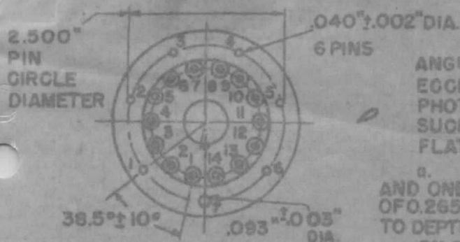
ENLARGED BOTTOM VIEW
