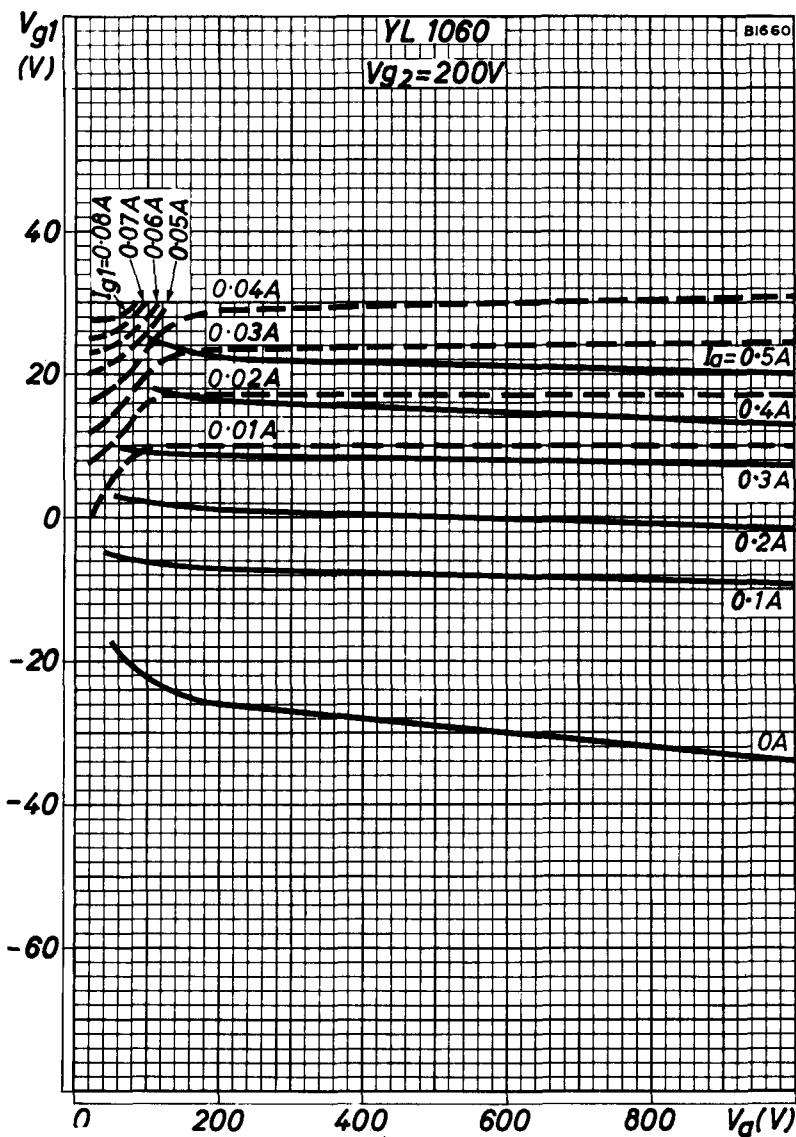
CONSTANT CURRENT CHARACTERISTICS V_{g2} = 200V
