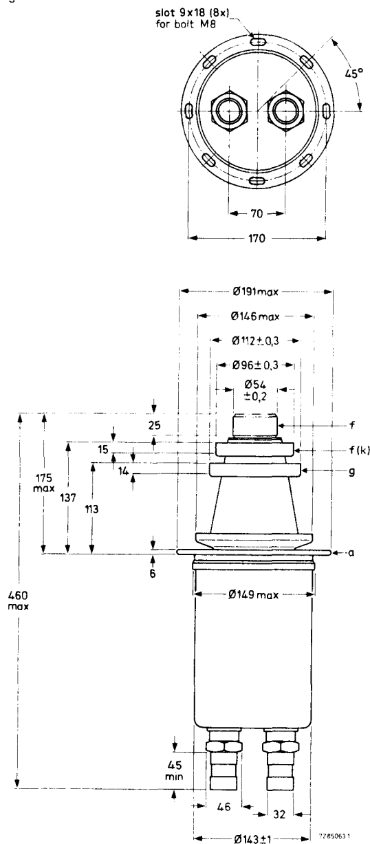
Fig. 1 Mechanical outline.
