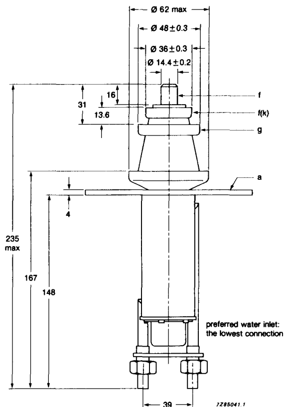
Fig. 2 Mechanical outline – YD1162.
