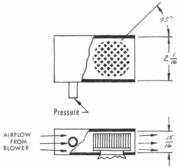
- COWLING DETAIL -
