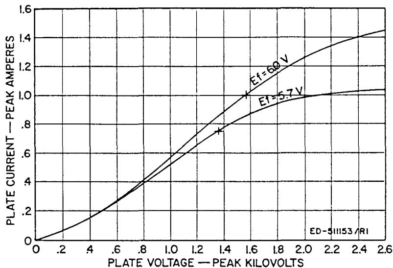
PLATE CURRENT CHARACTERISTICS
