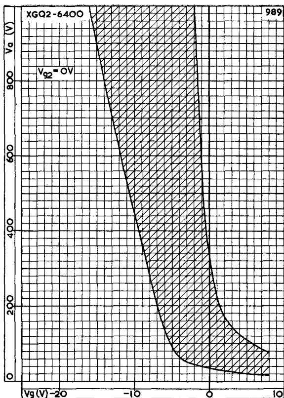
CONTROL CHARACTERISTIC
