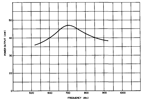
P-BAND OSCILLATOR
