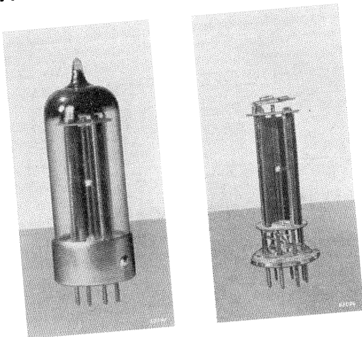
Fig. 1 The UY 41, showing the electrode system (approximately actual size).
