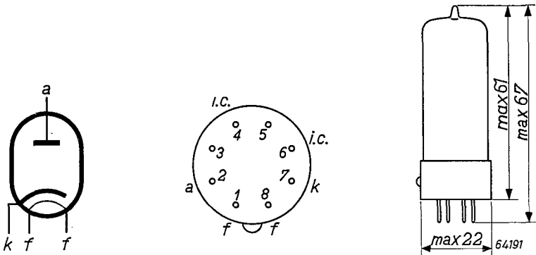
Fig. 3 Electrode arrangement, electrode connections and maximum dimensions in mm of the UY 41.
