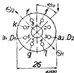
Fig. 2 Arrangement of electrodes and contacts.
