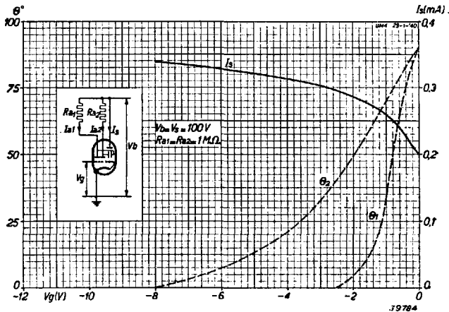
Fig. 5 Shadow angles \theta_1 and \theta_2 , measured at the edge of the screen, and screen current I_s as a function of grid voltage on a supply voltage of 100 V.
