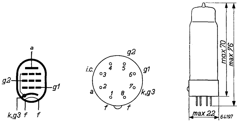
Fig. 3 Electrode arrangement, electrode connections and maximum dimensions in mm.
