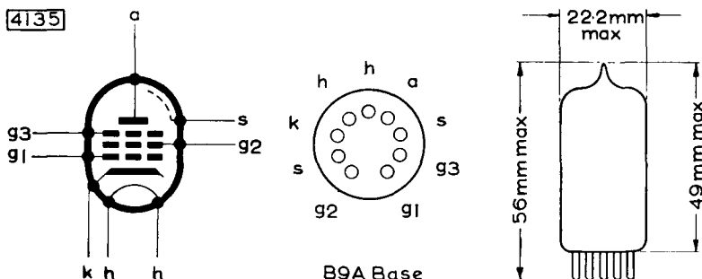
B9A Base
