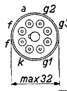
Fig. 2 Arrangement and sequence of con- tacts.
