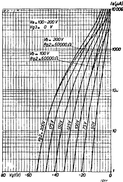
Fig 3 Anode current as a function of grid bias at V_a = 100 - 200 V and V_{g3} = 0 V, with screen voltage as parameter. The broken lines show the anode current when the valve is controlled, with the screen grid fed through a resistance of 60,000 Ohms from the 200 V or 100 V source.
