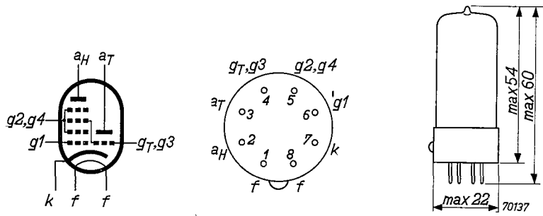
Fig. 2 Electrode arrangement, electrode connections and maximum dimensions in mm of the UCH 41.
