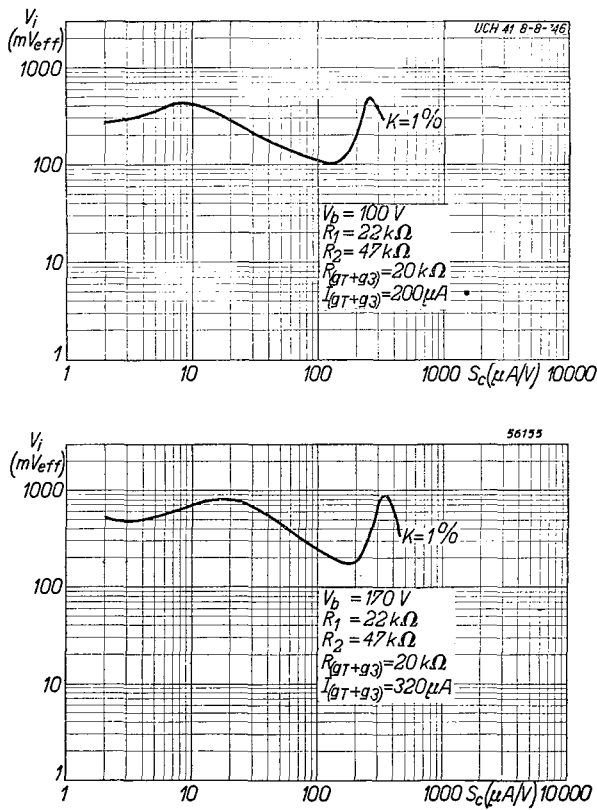
Fig. 14 The effective voltage ( V_i ) of an interfering signal at the control grid of the UCH 41, producing 1% cross modulation, as a function of the conversion conductance ( S_c ). Measurements taken in the circuit shown in Fig. 3. Upper figure: V_b=100 V ; lower figure: V_b=170 V .
