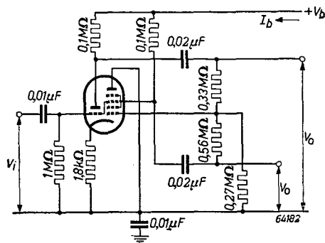
Fig. 4 The UCH 41 used as phase inverter.
