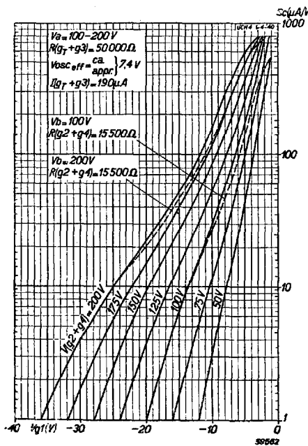
Fig. 5 Upper diagram; Maximum permissible effective value of R.F. alternating voltage at 1 % cross modulation ( K = 1\% ) and also for 1 % modulation hum ( mb = 1\% ), both in respect of the interfering signal at the grid, as a function of conversion conductance. Screen grid fed through a resistance of 15,500 ohms from the 100 V line. Lower diagram; Conversion conductance Sc , anode current I_a , screen grid current I(g_2 + g_4) , internal resistance R_i and equivalent noise resistance R_{eq} as a function of grid bias.
