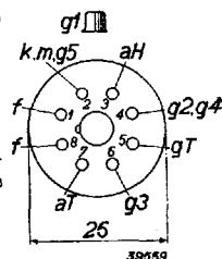
Fig. 2. Arrangement of electrodes and contacts.
