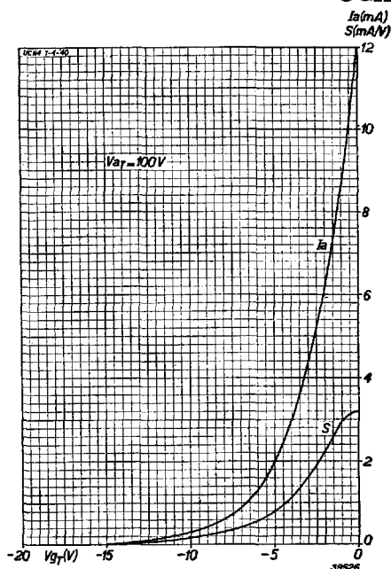
Fig. 15 Anode current and mutual conductance of the triode part as functions of the negative grid bias at V_{aT} = 100 V.
