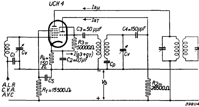
Fig. 17 Circuit diagram for employing the UCH 4 as mixer in AC/DC sets for a working voltage of 200 V.
