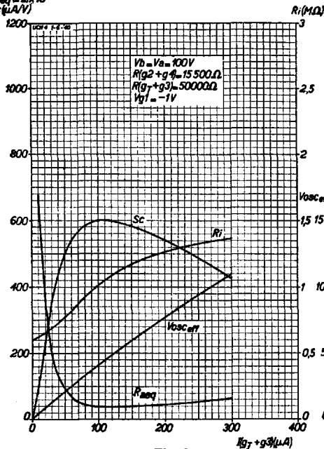
Fig. 6 Conversion conductance, internal resistance, alternating oscillator voltage and equivalent noise resistance as a function of oscillator current, with screen grid fed through a 15,500 Ohm resistance from 100 V, at V_{g_1} = -1V .
