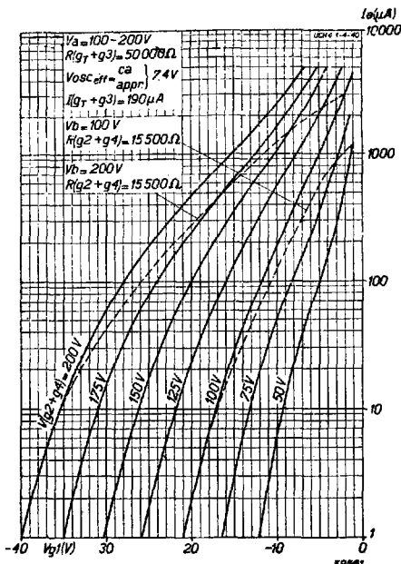
Fig. 3 Anode current as a function of grid bias at V_a = 100 - 200 V, R(g_1 + g_3) = 50,000 Ohms, I(g_1 + g_3) = 190 \mu A, with V(g_2 + g_4) as parameter.
