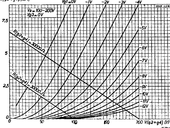
Fig. 16 Screen grid current as a function of screen voltage at Va = 100-200 V and Vg_3 = 0 V , with grid bias as parameter.
