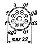
Fig. 2 Arrangement and sequence of connections.
