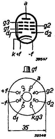
Fig. 2 Arrangement of electrodes and contacts
