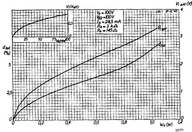
Fig. 7. Total distortion and alternanting grid voltage as a function of output power at V_a = V_{g2} = 100 V.
