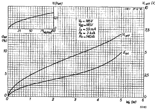
Fig. 8. Total distortion and alternanting grid voltage as a function of output power at V_a = V_{g2} = 185 V.
