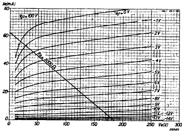
Fig. 4 Anode current as a function of anode voltage at V_{g2} = 100 V, with V_{g1} as parameter.
