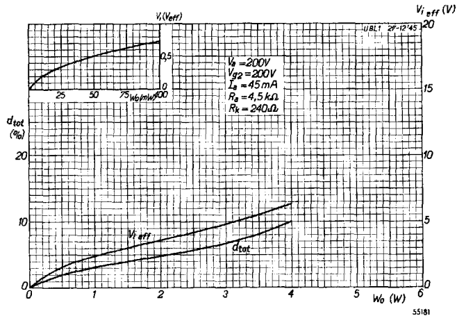
Fig. 9 Total distortion and alternanting grid voltage as a function of output power at V_a = V_{g2} = 200 V, for 9 W operation
