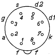
Fig. 2 Electrode arrangement, electrode connections and dimensions in mm of the UBC 41.
