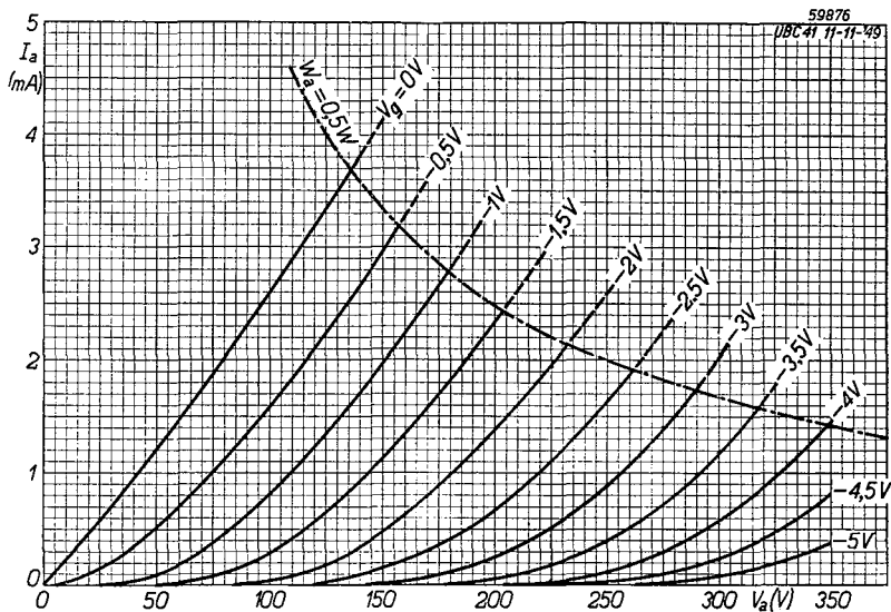
Fig. 5 I_a/V_a characteristics of the UBC 41. The dot-dash line indicates the maximum permissible anode dissipation ( W_a = 0.5W ). For the diode characteristics see Figs. 6 and 7 in the description of the EBC 41.
