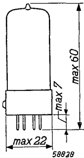
Fig. 2 Electrode arrangement, electrode connections and dimensions in mm of the UBC 41.
