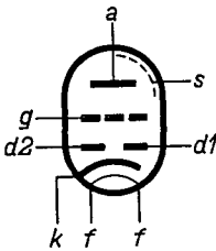
Fig. 2 Electrode arrangement, electrode connections and dimensions in mm of the UBC 41.
