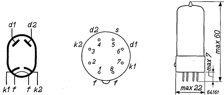
Fig. 2 Electrode arrangement, electrode connections and dimensions in mm of the UB 41.
