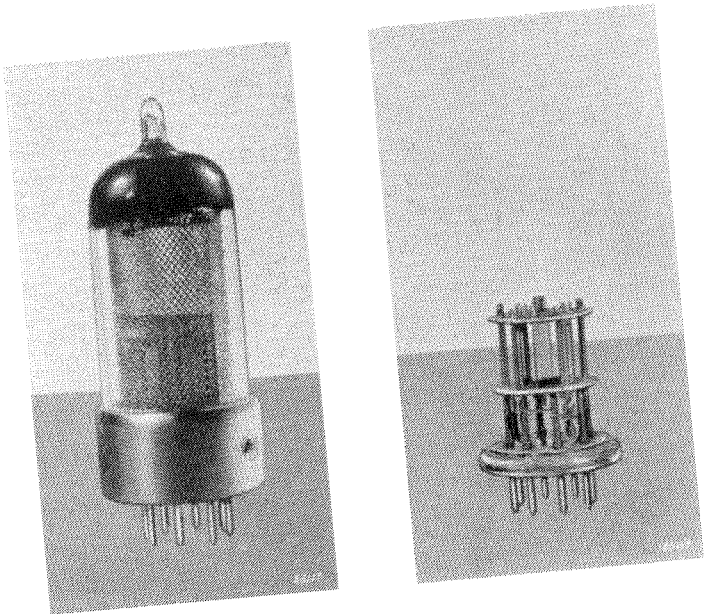
Fig. 1 The UB 41, showing the electrode system (envelope and screening cage removed; approximately actual size).
