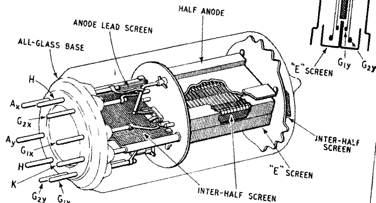
Constructional details of the UA-55 valve and (top right) section showing arrangement of electrodes
