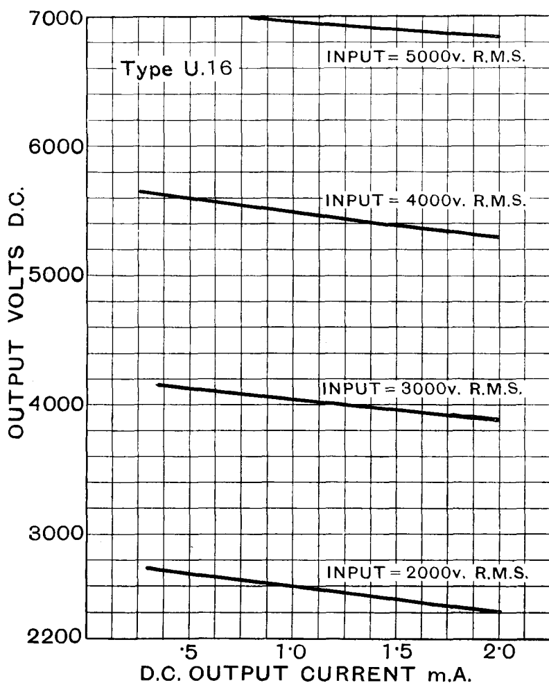
CHARACTERISTIC CURVES OF AVERAGE VALVE.
