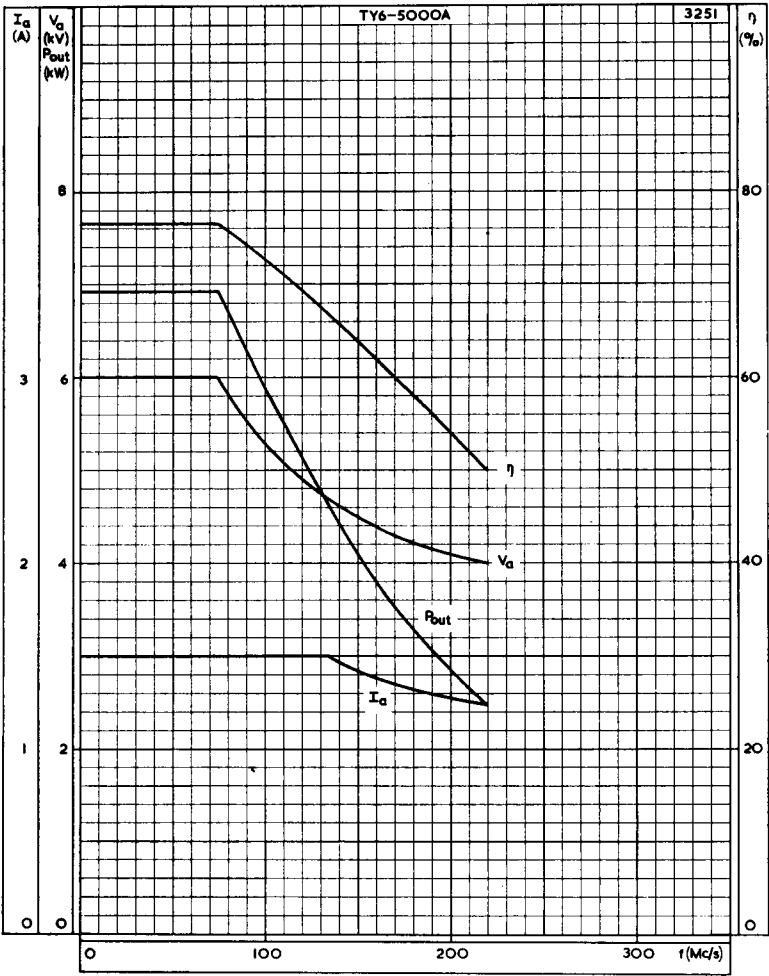
FREQUENCY CHARACTERISTICS
