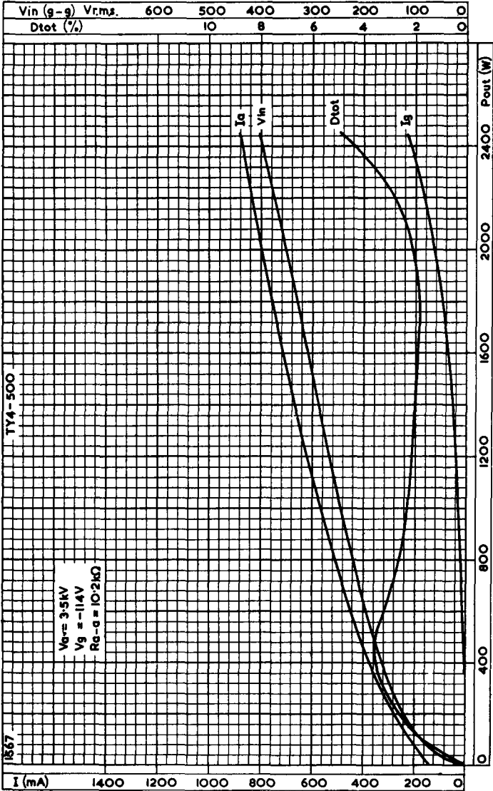
TWO VALVES AS CLASS "B" A.F. AMPLIFIER. V_a = 3.5 \text{ kV}
