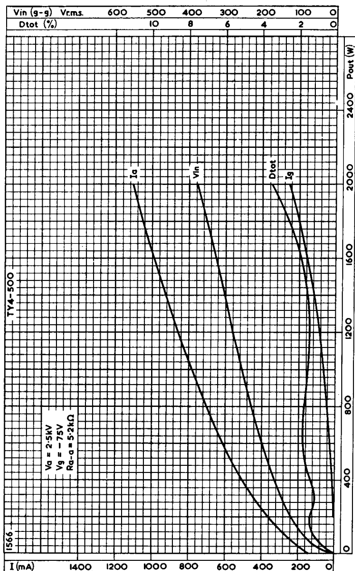
TWO VALVES AS CLASS "B" A.F. AMPLIFIER. V_a = 2.5 \text{ kV}
