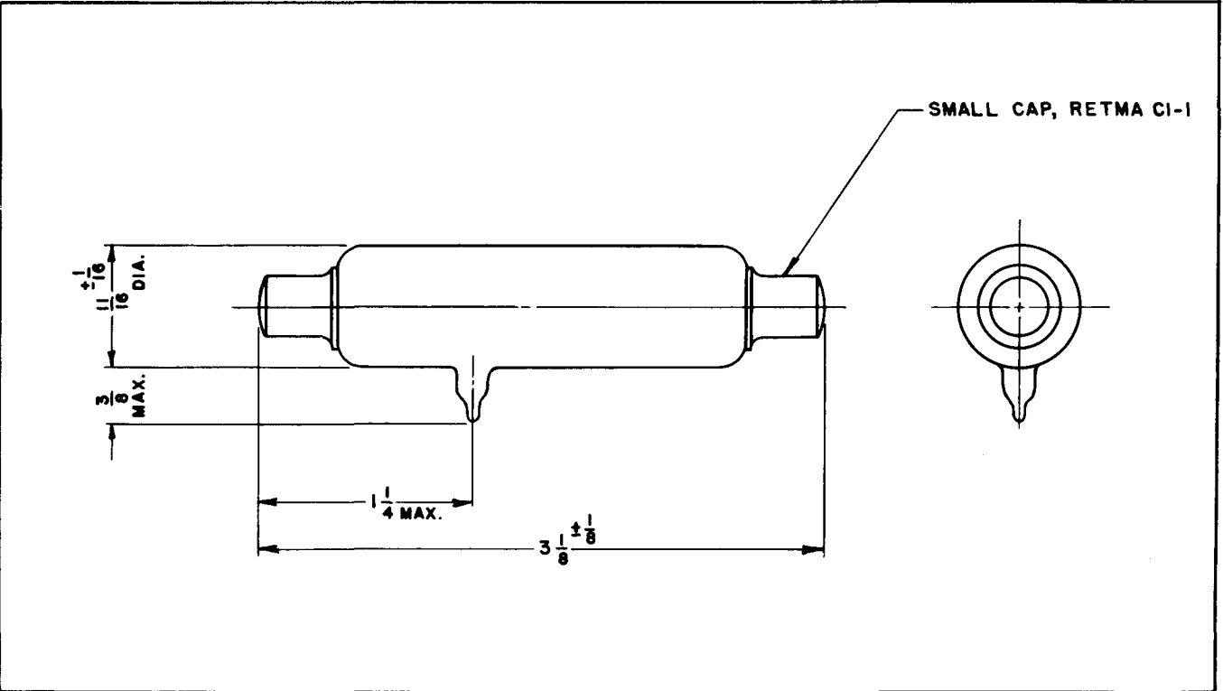
OUTLINE DRAWING
