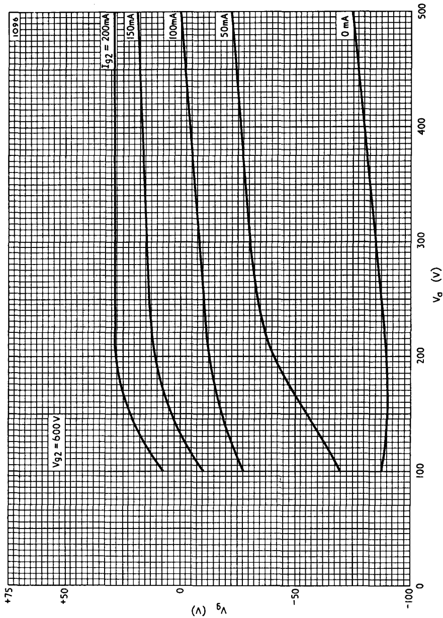
Fig. 6. Constant screen current curves at V_{g2} = 600 \text{ V} .
