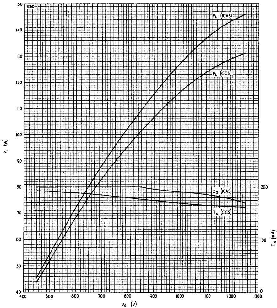
Fig. 12. Class C telegraphy. Power output/anode voltage curves.
