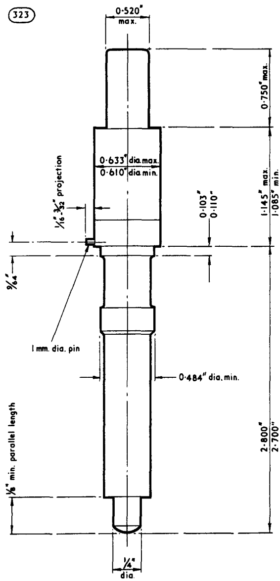
Fig. 2. Outline drawing.
