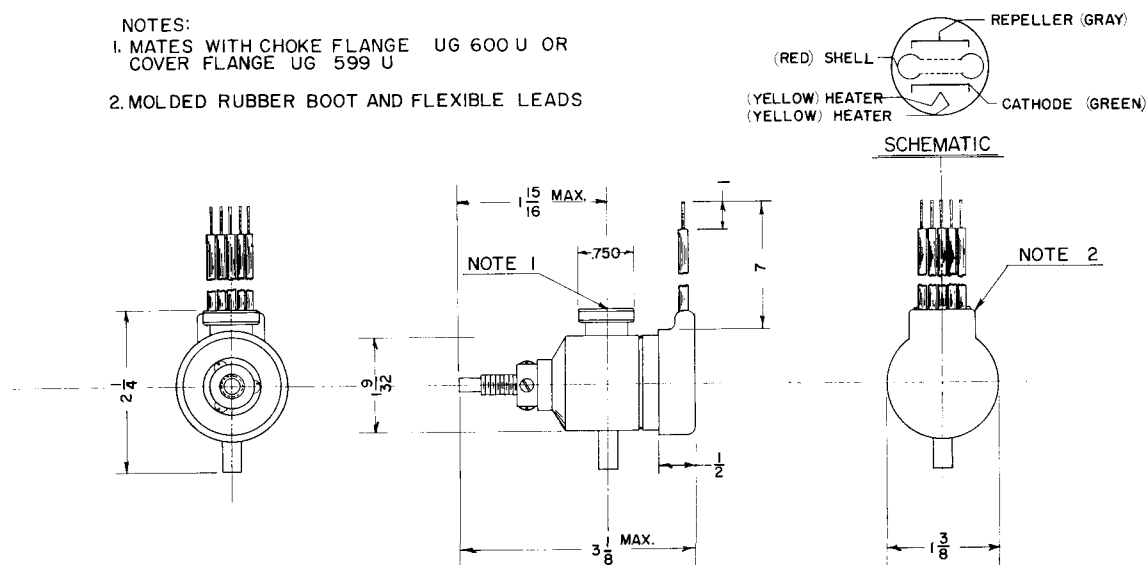
OUTLINE DRAWING
