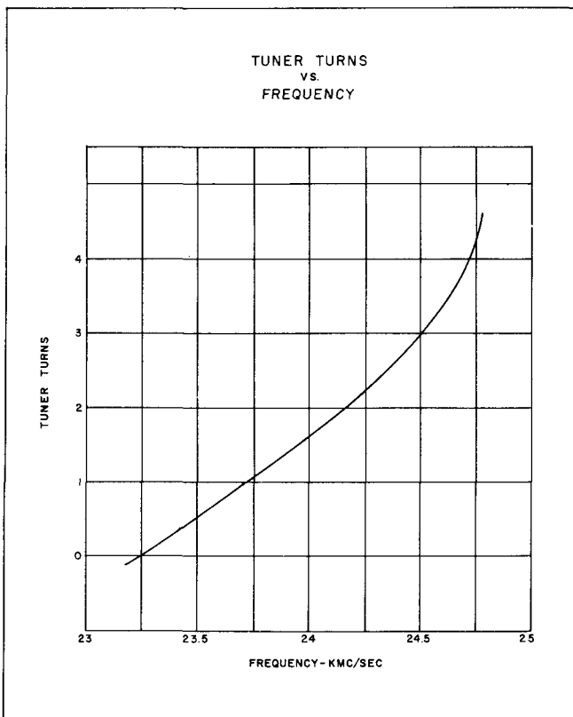
TUNER TURNS VS. FREQUENCY
