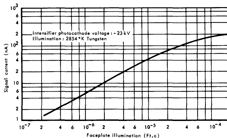
Fig 2 - Light transfer characteristic.
