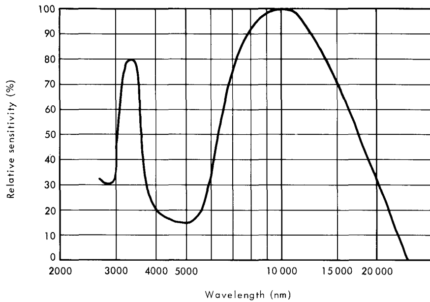
Figure 1 - Spectrale response.
