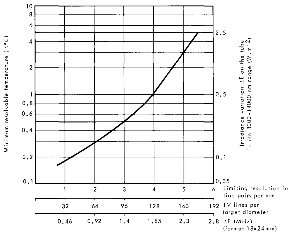
Figure 4 - Minimum resolvable temperature in panning mode ( v = 0.4 \text{ cm.s}^{-1} ) Black body near to ambient temperature - F/1 aperture number.
