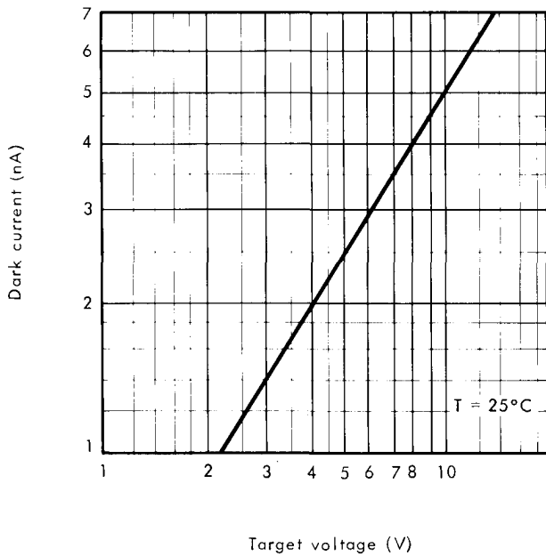
Figure 3 - Dark-current characteristics.
