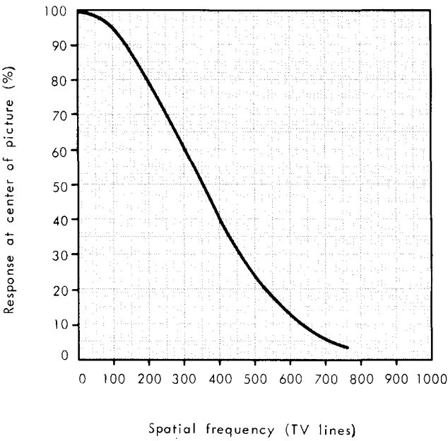
Figure 7 - Typical MTF characteristics with a 100 % contrast vertical bar test pattern.
