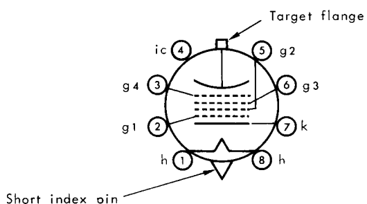
BASING DIAGRAM
