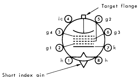
BASING DIAGRAM
