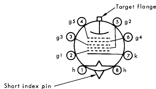
BASING DIAGRAM
