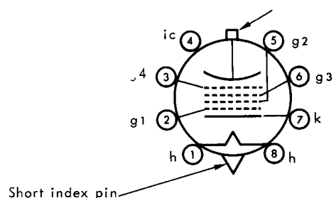
BASING DIAGRAM
