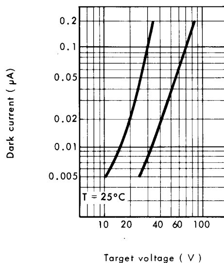
RANGE OF DARK CURRENT Scanned area of photoconductive layer 12.7 mm x 9.5 mm
