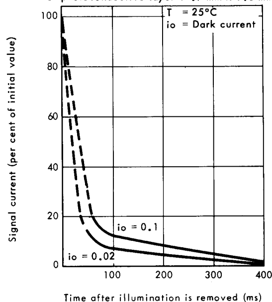
TYPICAL PERSISTENCE CHARACTERISTICS Initial highlight signal current of 0.2 \mu\text{A} scanned area of photoconductive layer 12.7 mm x 9.5 mm
