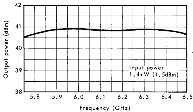
FIGURE 2 - Frequency response
