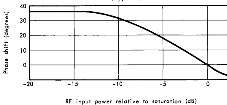
PHASE SHIFT VERSUS RF DRIVE (typical)
