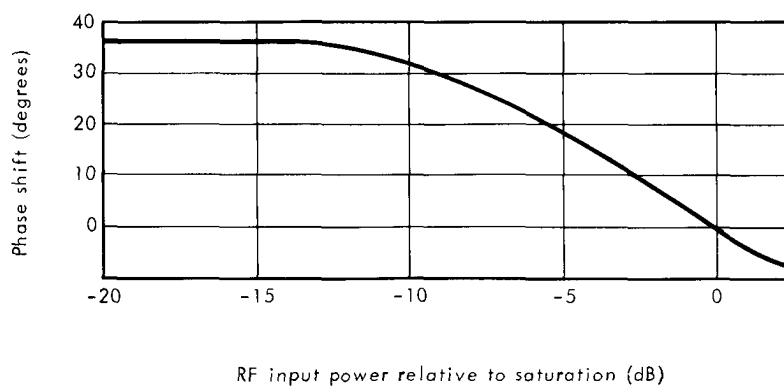
PHASE SHIFT VERSUS RF DRIVE (Typical)
