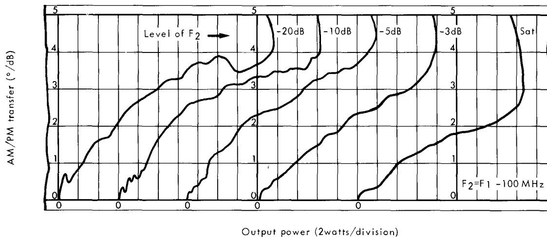
PHASE SHIFT VERSUS RF DRIVE (Typical)
