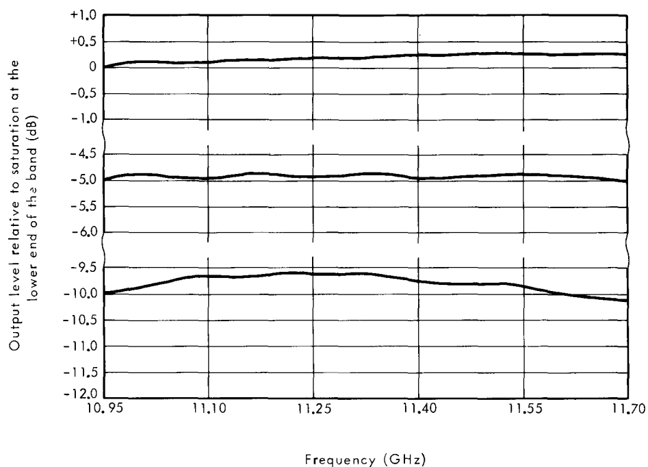
AM/PM TRANSFER VERSUS OUTPUT POWER (level of F_1 held constant while level of F_2 is varied)
