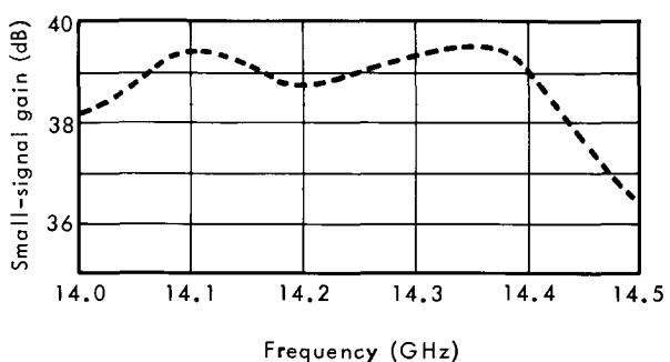
Fig. 2 - Variations of small-signal gain versus frequency (typical).
