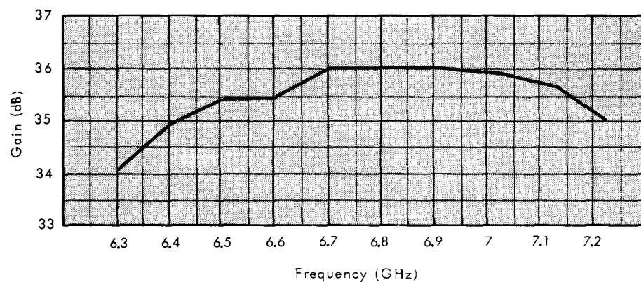
FIGURE 3 - Gain flatness at saturation.
