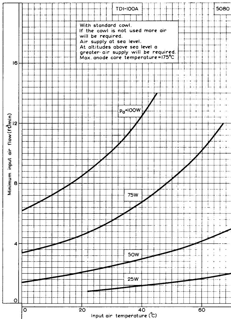
MINIMUM INPUT AIR FLOW PLOTTED AGAINST INPUT AIR TEMPERATURE
