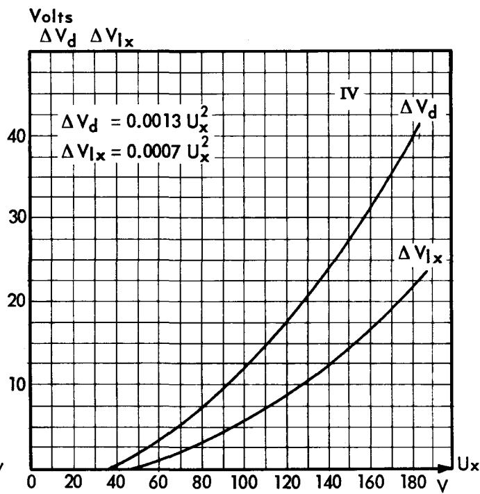
Dynamic correcting voltages \Delta V_d and \Delta V_{lx} versus x deflecting voltage U_x .
