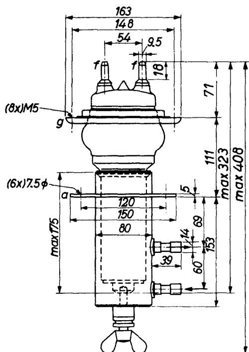
Fig. 1 Mechanical outline.
