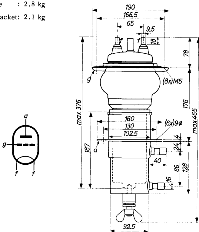
Fig. 2 Mechanical outline.
