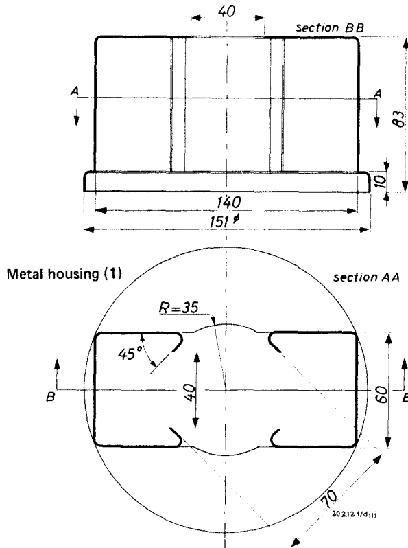
Fig. 2 Cooling device details.
